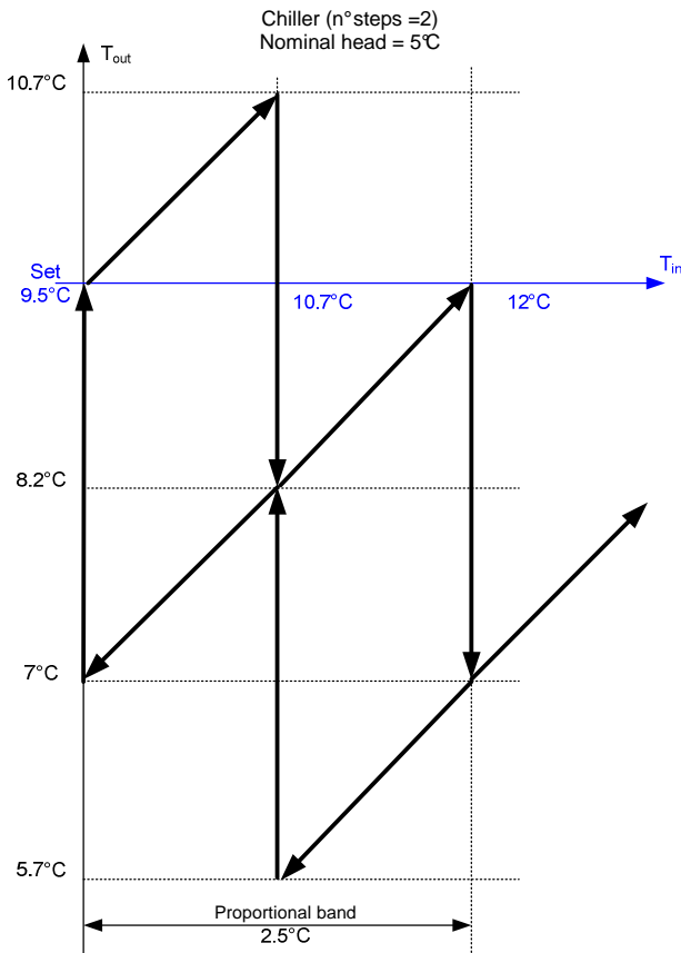
Figure 1.6.1.c: Relationship between T_{in} and T_{out} , with 2 steps (chiller)
