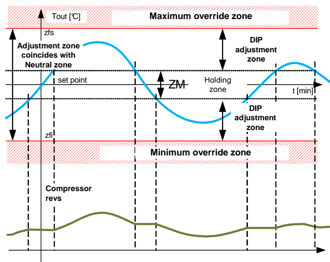
Figure 1.6.5.m: operating diagram of DIP adjuster output
