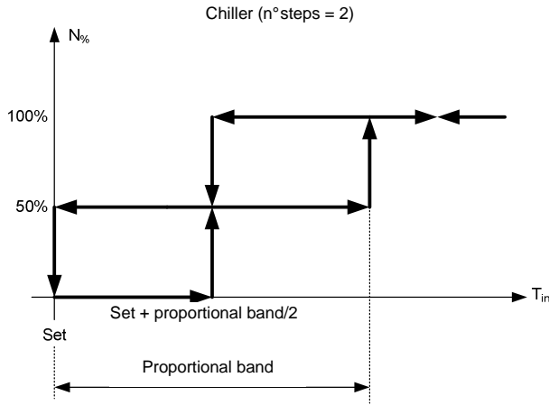
Figure 1.6.1.a: T_{in} is the input variable, N_{\%} is the n° of active steps expressed in % (chiller)
