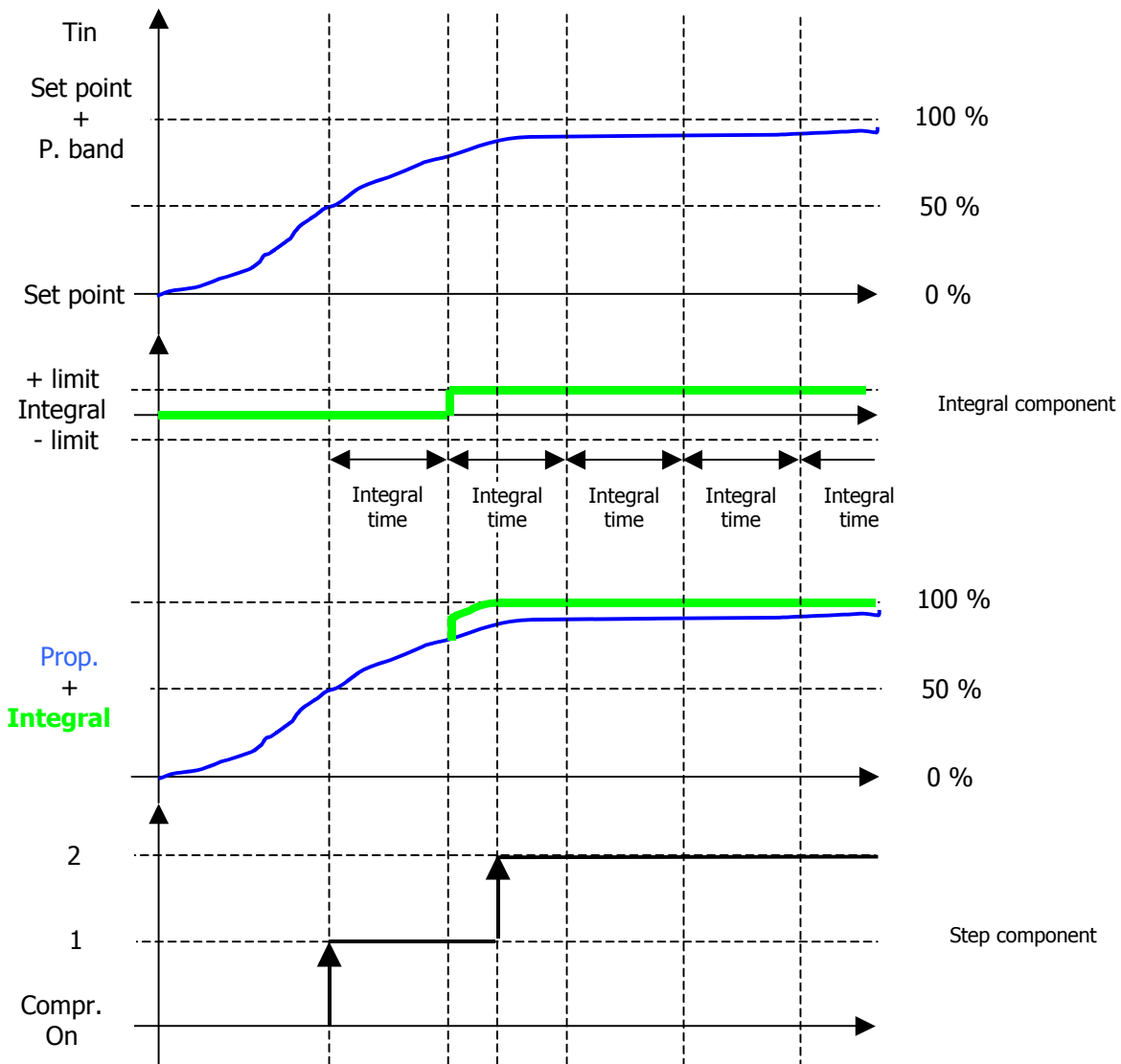
Fig 1.6.2.e: Example of a 2 step adjustment in the chiller mode
