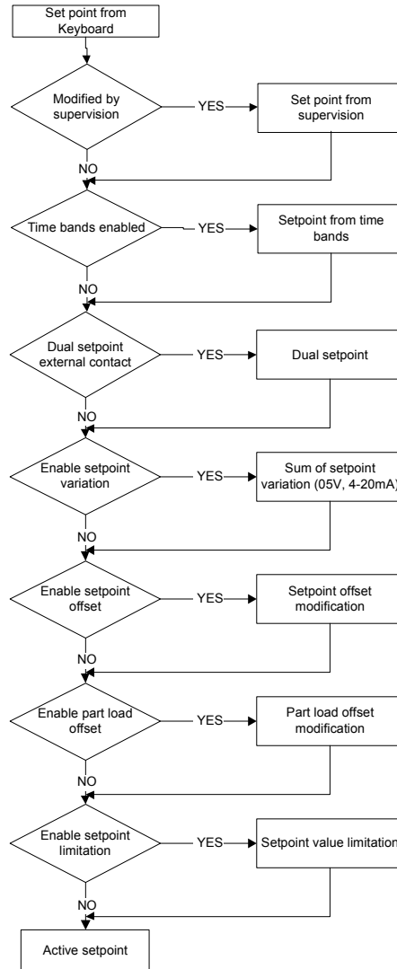
Figure 1.7.a: sequence of the setpoint modification functions set to obtain the active setpoint.
