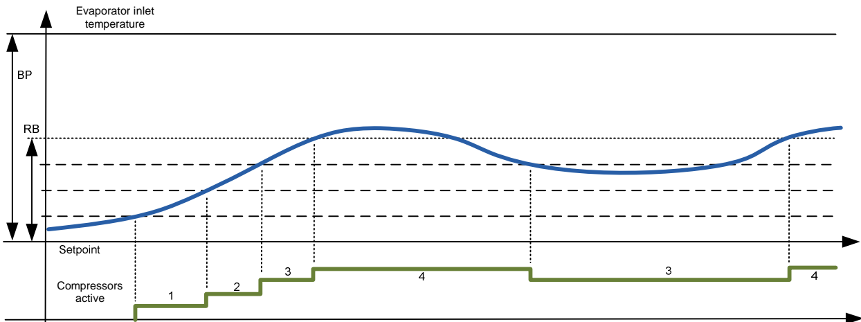
Figure 1.6.5.k: proportional adjustable with flexible steps on the inlet probe with offset = 0 and Rb = 50\%
