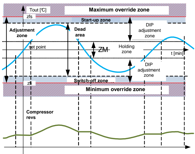
Figure 1.6.6.o: operating diagram of DIP adjuster output
