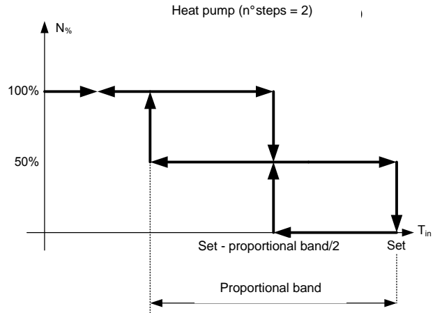
Figure 1.6.1.b: T_{in} is the input variable, N_{\%} is the number of active steps expressed in % (heat pump)
