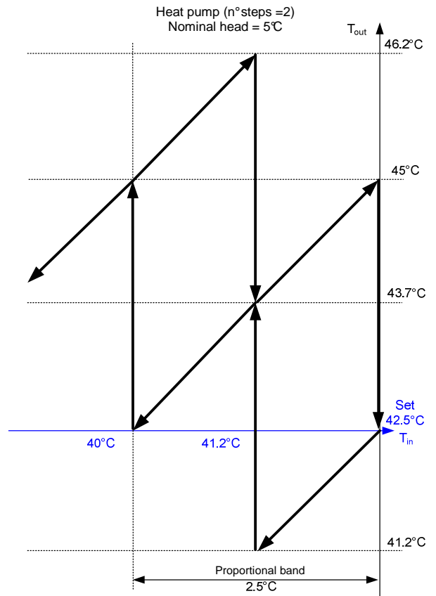
Figure 1.6.1.d: Relationship between T_{in} and T_{out} , with 2 steps (heat pump)
