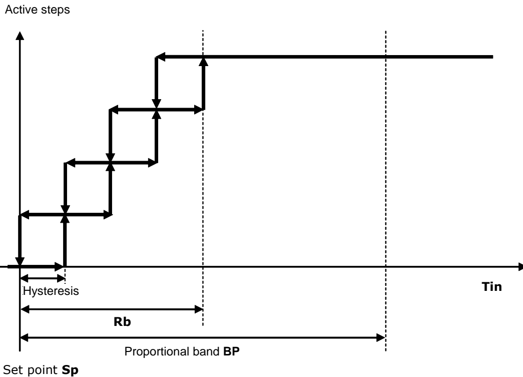
Figure 1.6.5.j: proportional step adjuster with offset = 0 and Rb = 50\%
