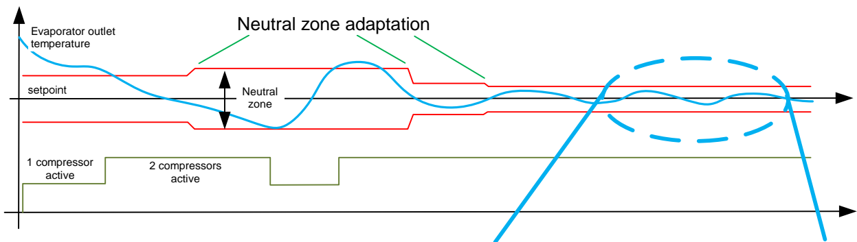
Figure 1.6.6.n: Neutral zone adjustment on outlet probe
