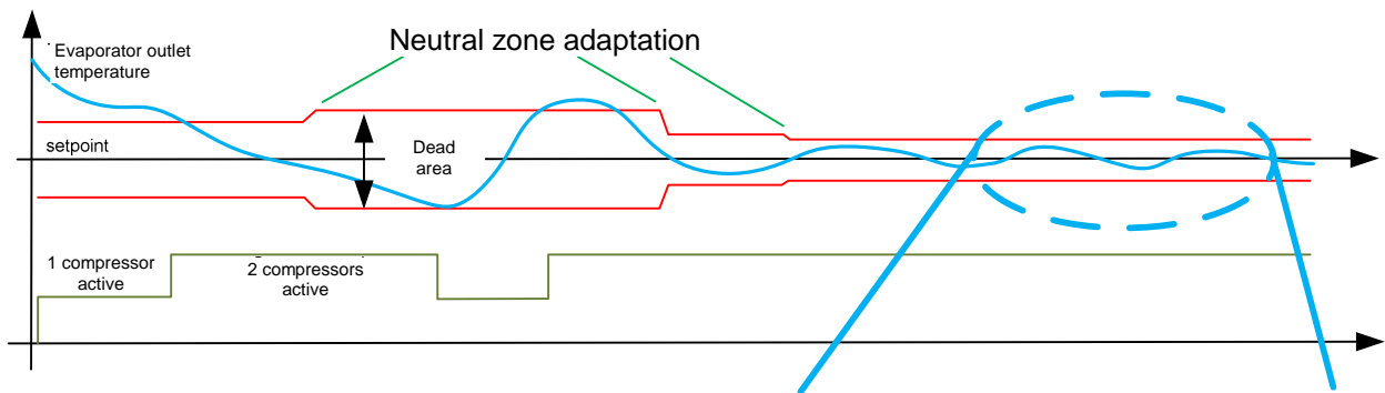
Figure 1.6.4.h: modulating adjustment on the outlet probe
