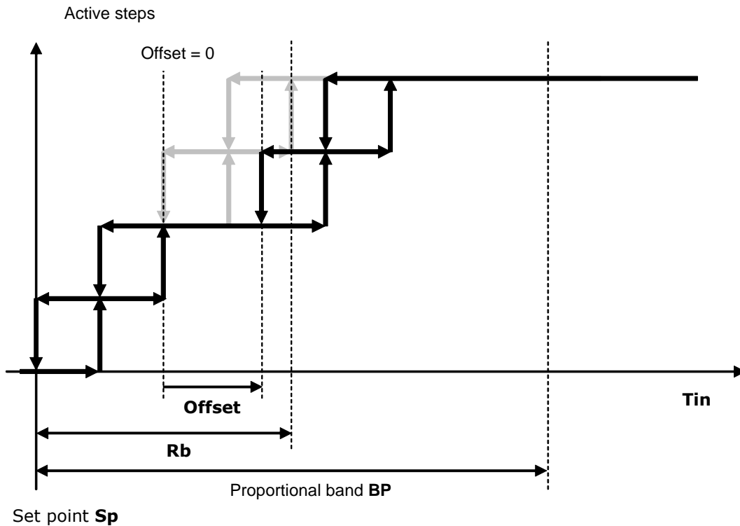
Figure 1.6.5.l: proportional step adjuster with offset > 0 and Rb = 50%
