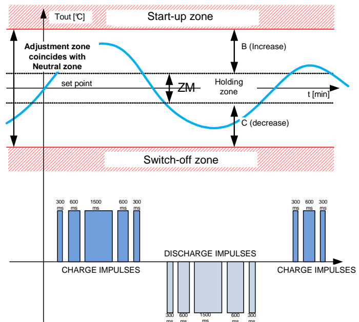
Figure 1.6.4.i: modulating adjustment for screw compressors
